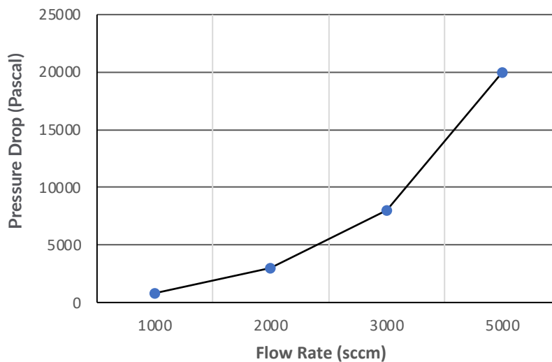
Pressure Drop of the PMF2000/PMFc3000
